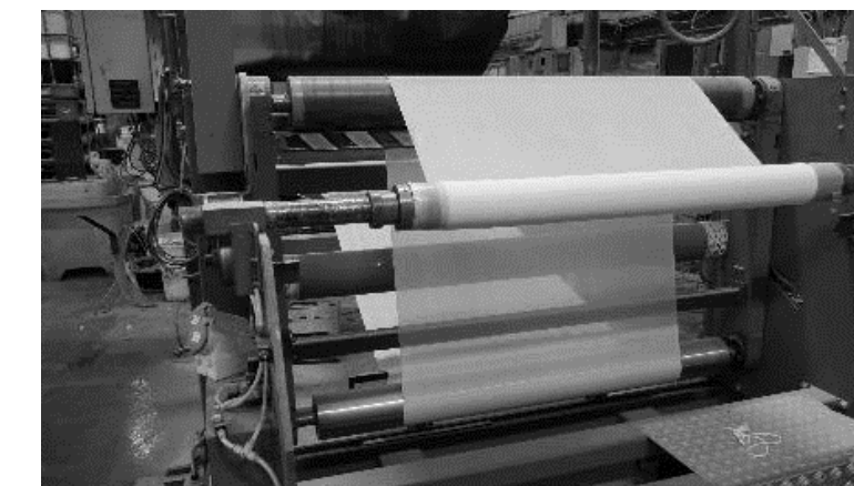
PVA Coating
